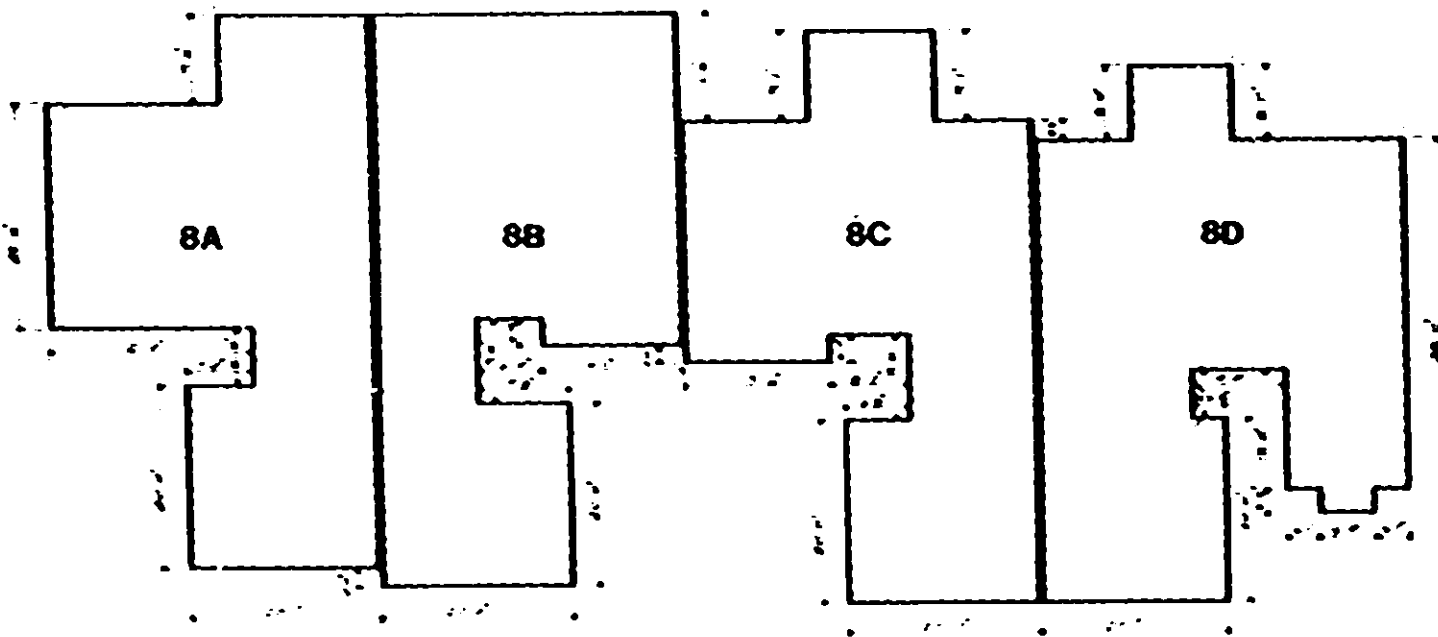
FOUNDATION PLAN
